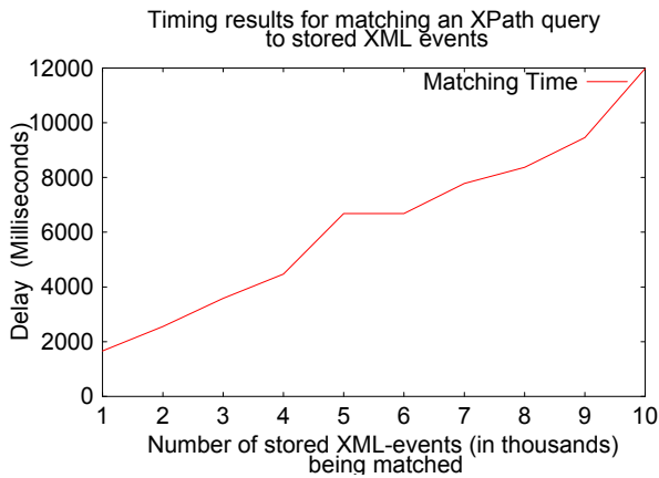
Figure 3: Matching XML-events
